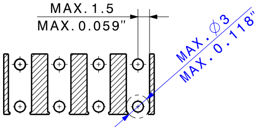
PASTE-FREE AREA
