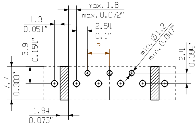
PASTE-FREE AREA
