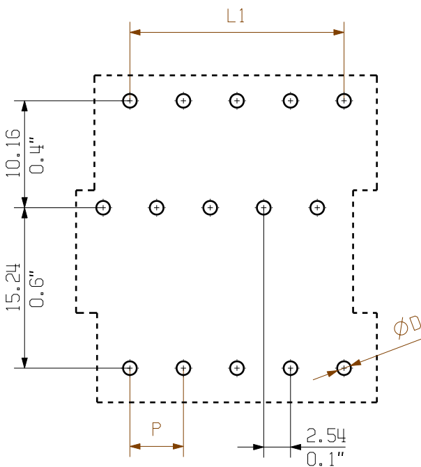
PCB LAYOUT
