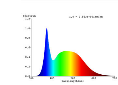
RGBW Remote Lamp 6500K
