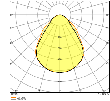
PL CMFT 600 P 30W 865 U19 PS
