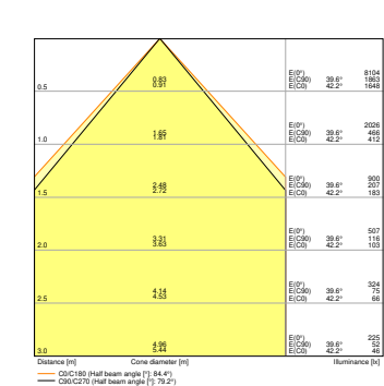
PL CMFT 600 P 30W 865 U19 PS
