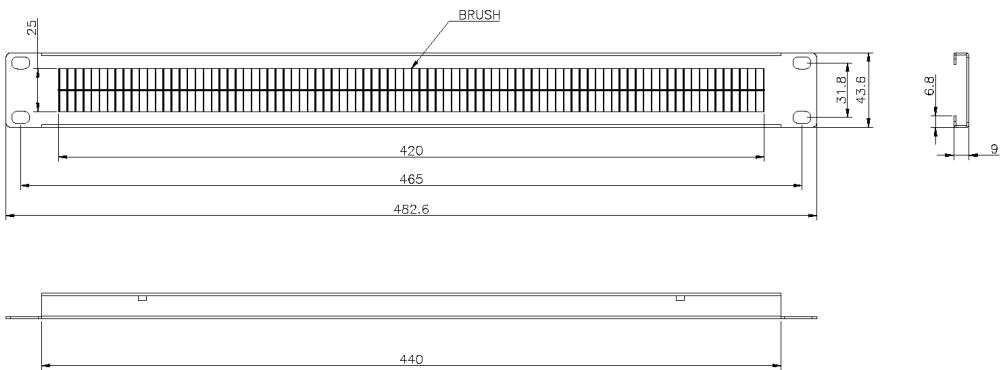
Product drawing (100-595)
