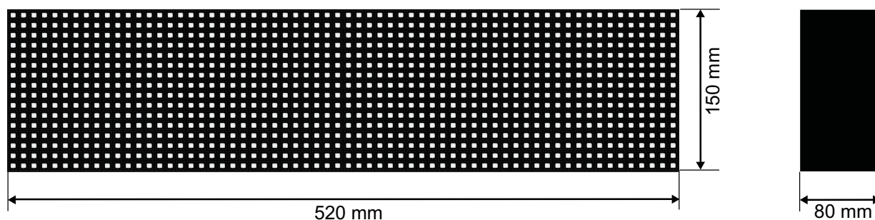
Fig. 2 DISBRSE dimensions
