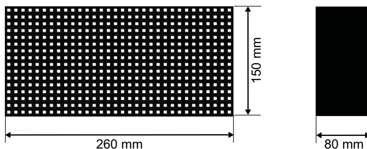
Fig. 1 DISARSE dimensions
